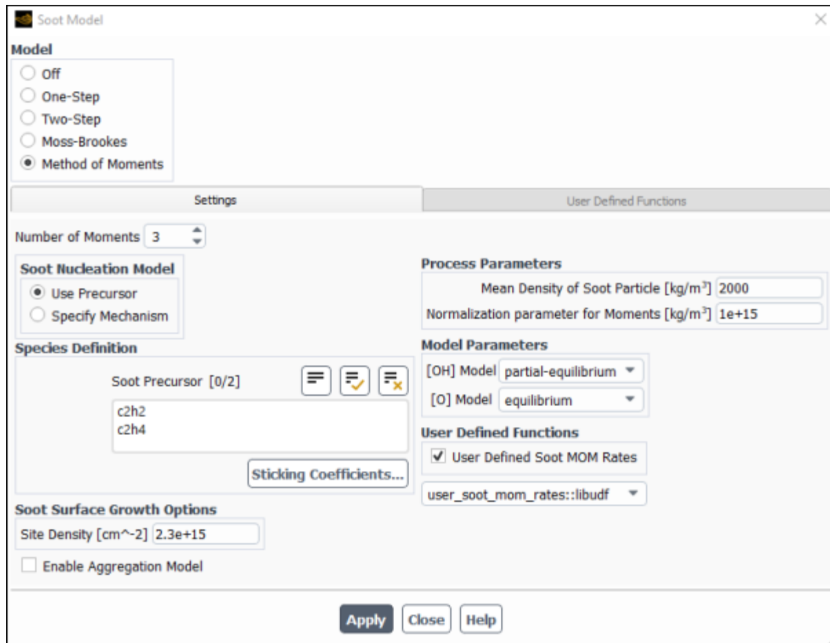
Figure 6.62: The Soot Model Dialog Box (User-Defined Soot MOM Rates)
