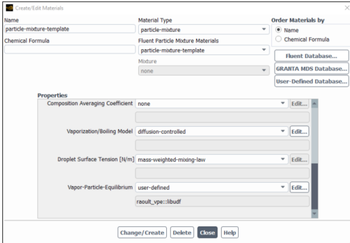
Figure 6.109: The Create/Edit Materials Dialog Box
