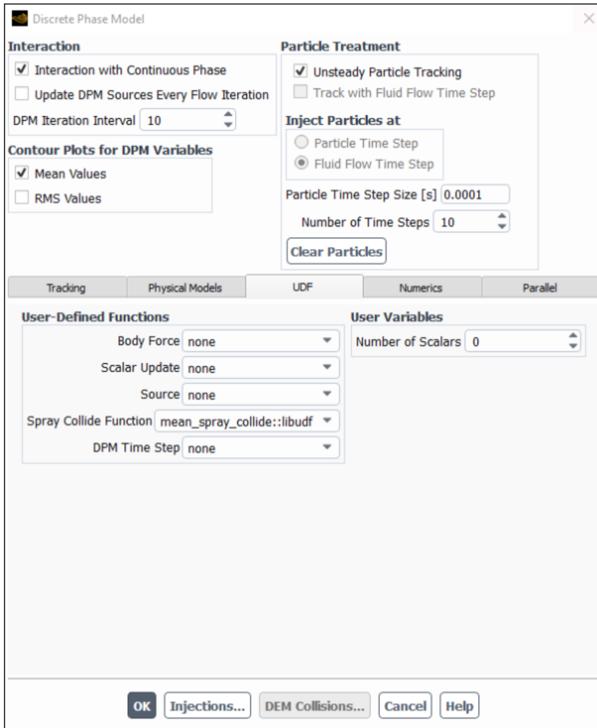
Figure 6.106: The Discrete Phase Model Dialog Box
