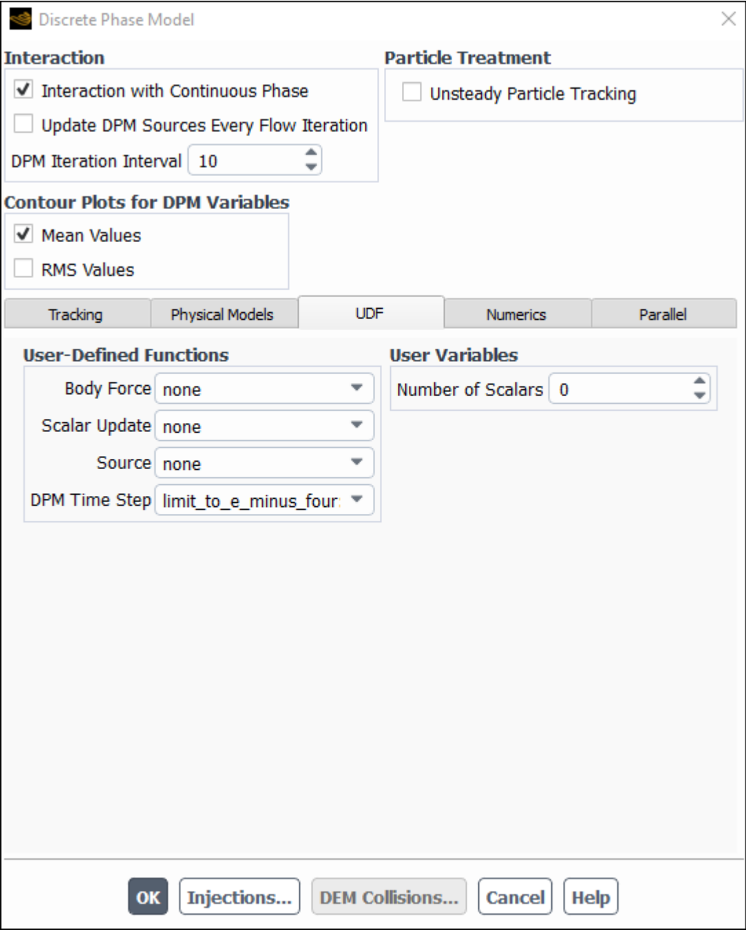
Figure 6.108: The Discrete Phase Model Dialog Box
