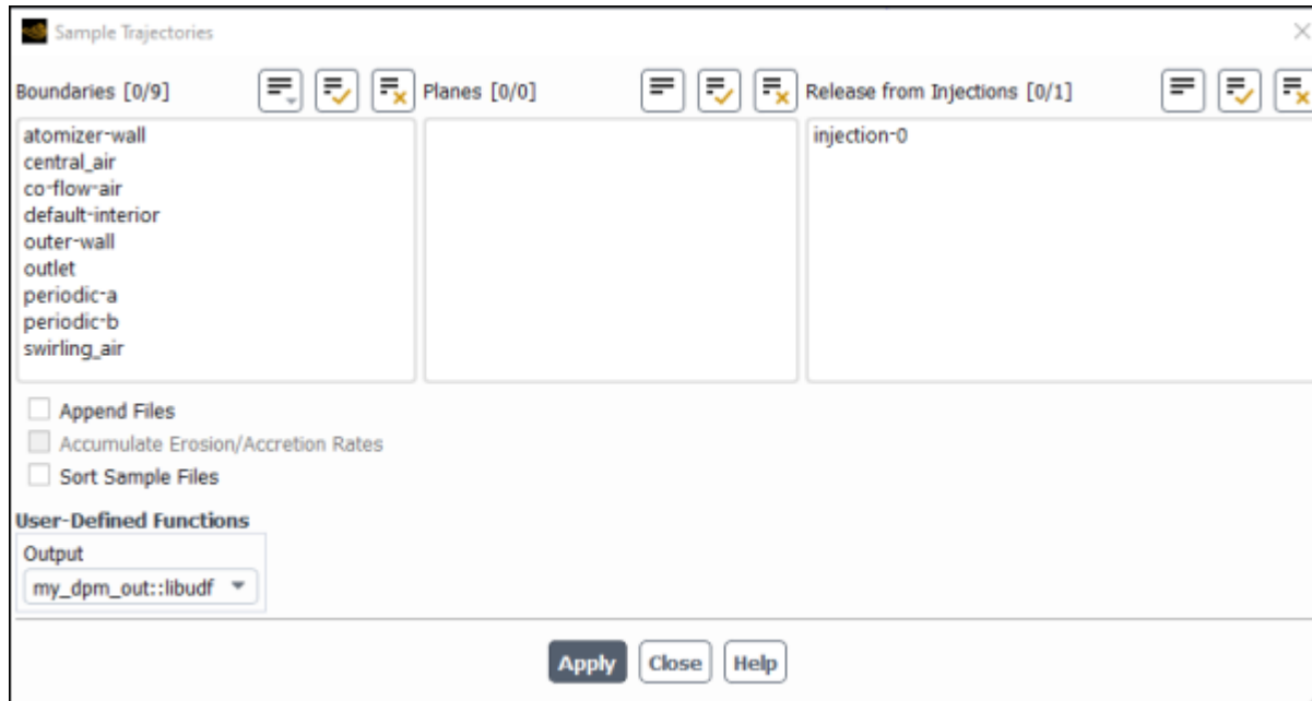
Figure 6.101: The Sample Trajectories Dialog Box
