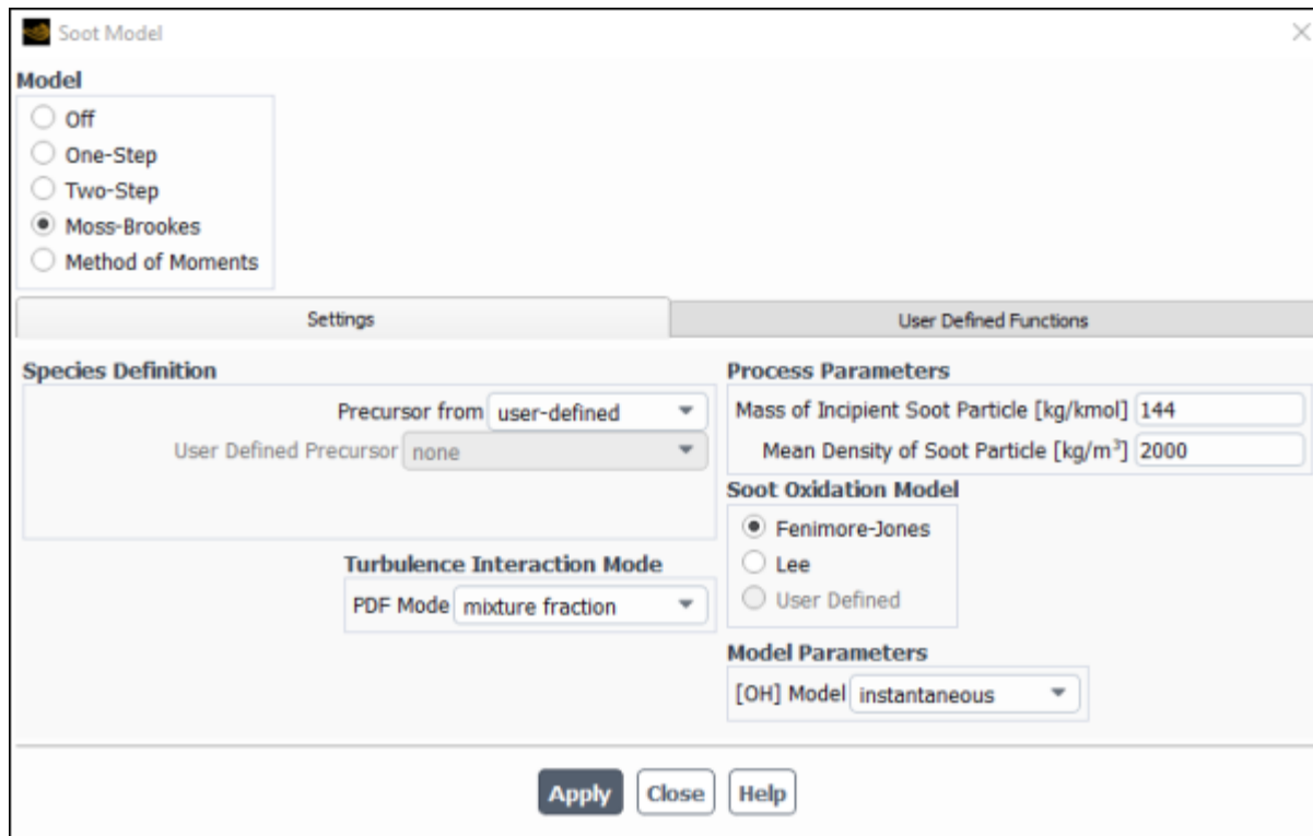
Figure 6.64: The Soot Model Dialog Box (User-Defined Precursor)
