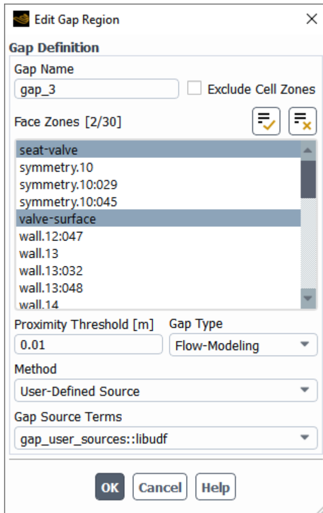
Figure 6.31: The Edit Gap Region Dialog Box
