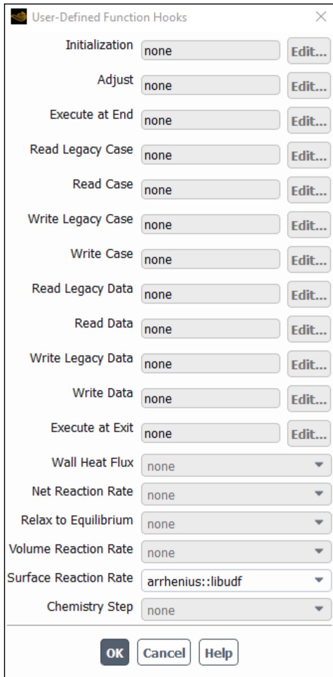
Figure 6.68: The User-Defined Function Hooks Dialog Box
