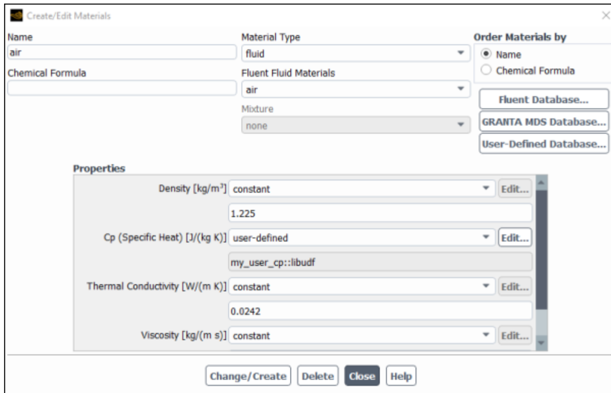
Figure 6.66: The Create/Edit Materials Dialog Box
