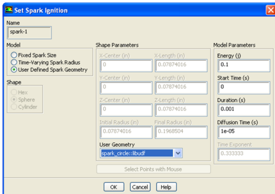
Figure 6.65: The Set Spark Ignition Dialog Box
