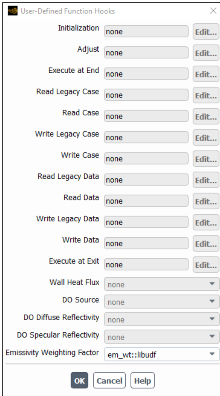
Figure 6.29: The User-Defined Function Hooks Dialog Box
