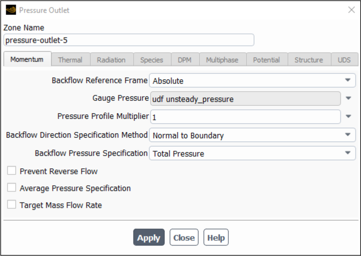
Figure 8.16: The Pressure Outlet Dialog Box
