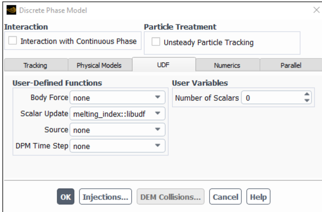
Figure 6.104: The Discrete Phase Model Dialog Box
