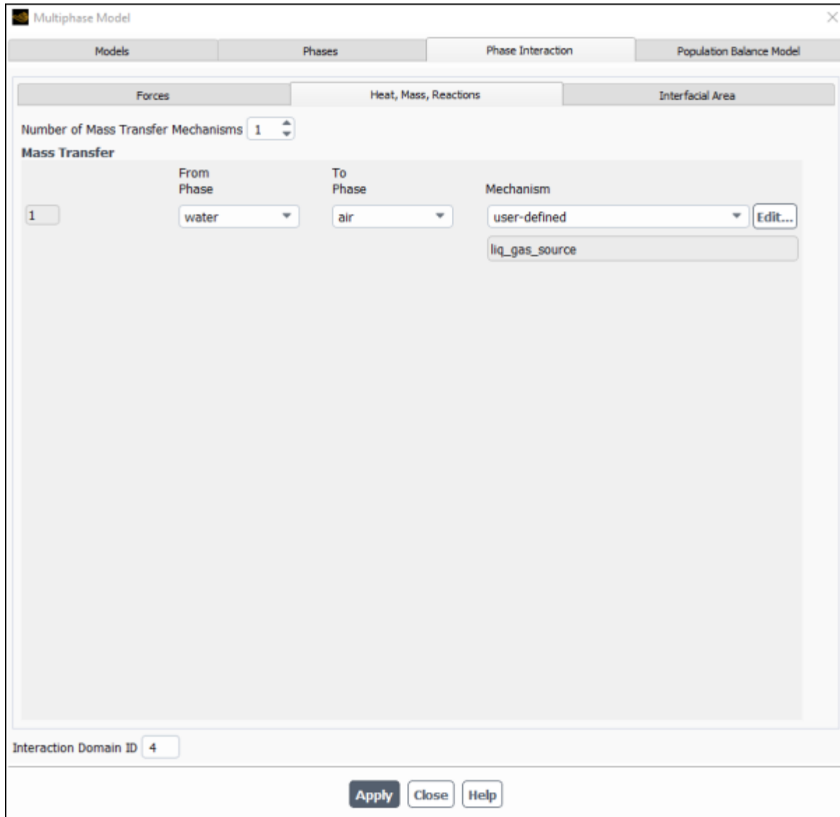
Figure 6.90: The Multiphase Model Dialog Box - Heat, Mass, Reactions Tab
