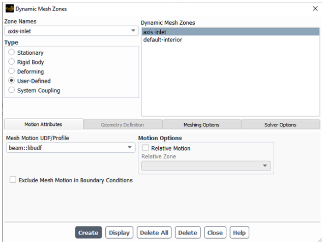
Figure 6.118: Dynamic Mesh Zones Dialog Box
