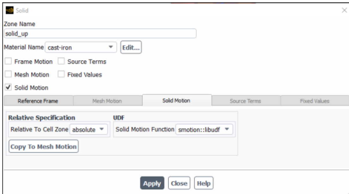
Figure 6.83: The Solid Dialog Box for Solid Motion
