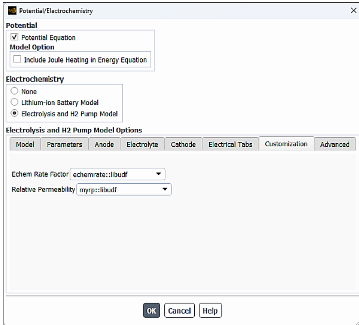
Figure 6.28: The Potential/Electrochemistry Dialog Box - Customization Tab
