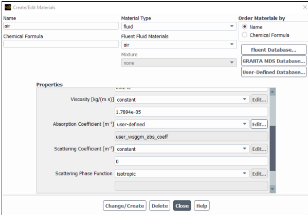
Figure 6.79: The Create/Edit Materials Dialog Box
