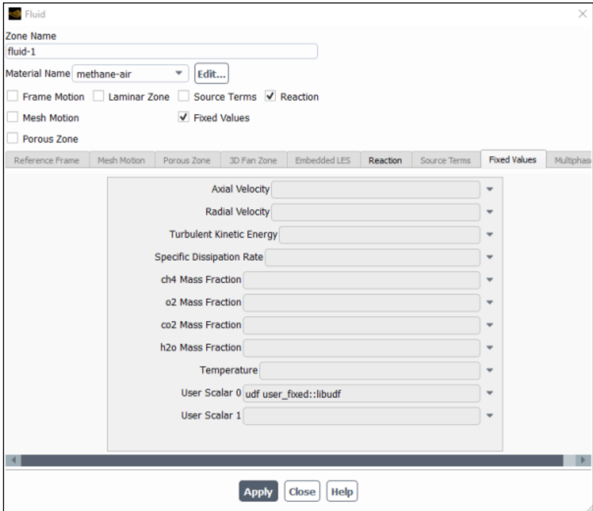
Figure 6.46: The Fluid Dialog Box with Fixed Value Inputs for User-Defined Scalars
