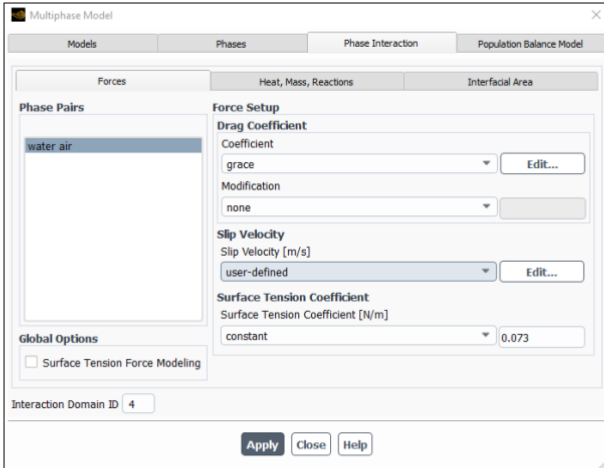
Figure 6.92: The Multiphase Model Dialog Box - Force Tab
