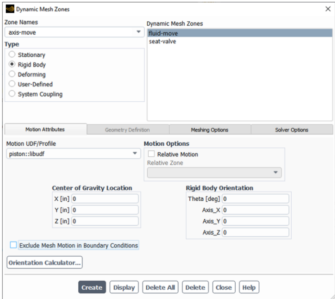
Figure 6.114: The Dynamic Mesh Zones Dialog Box
