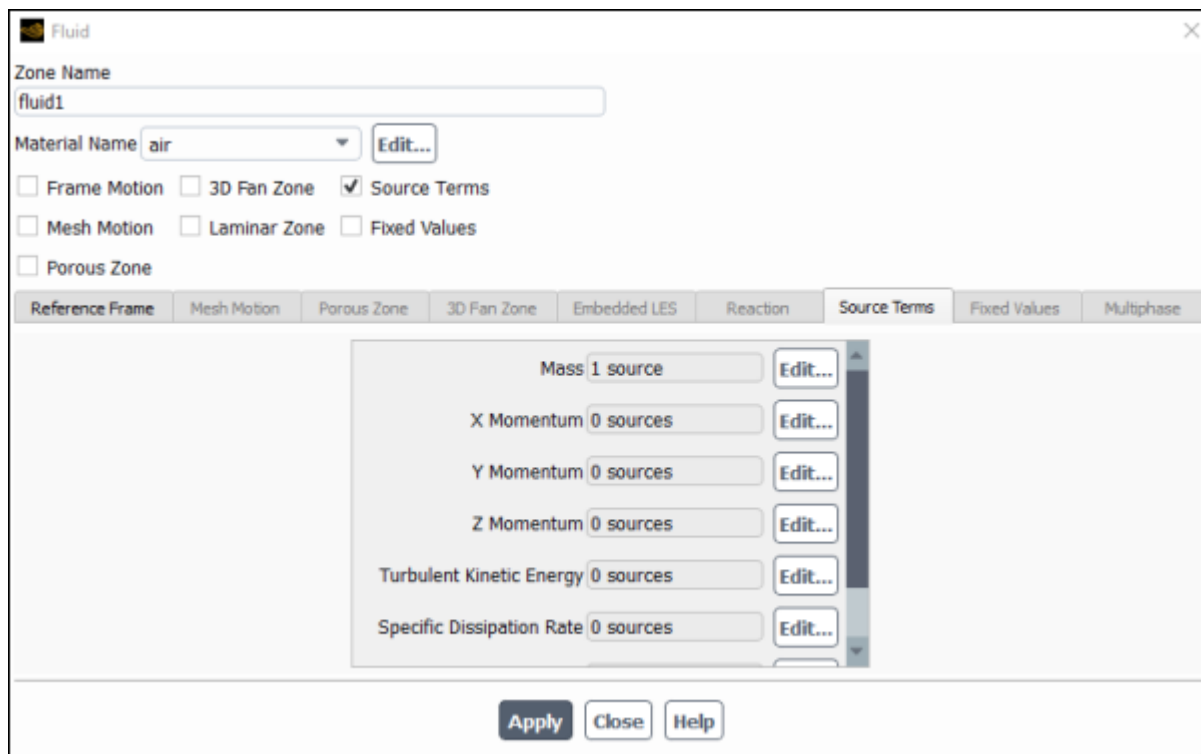
Figure 6.59: The Fluid Dialog Box
