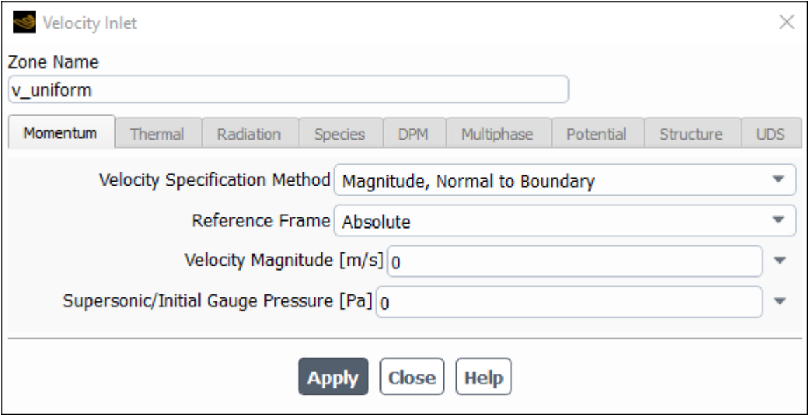
Figure 8.13: The Velocity Inlet Dialog Box
