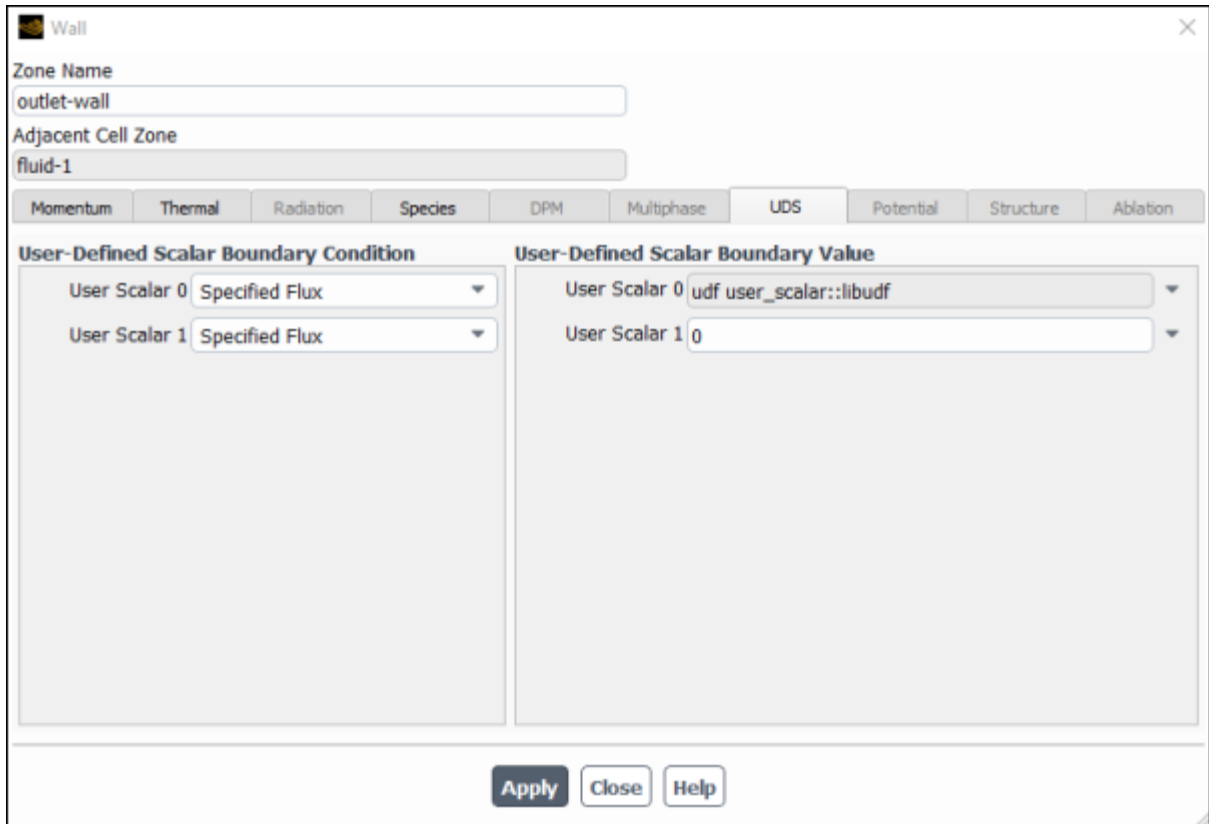
Figure 6.47: The Wall Dialog Box with Inputs for User-Defined Scalars
