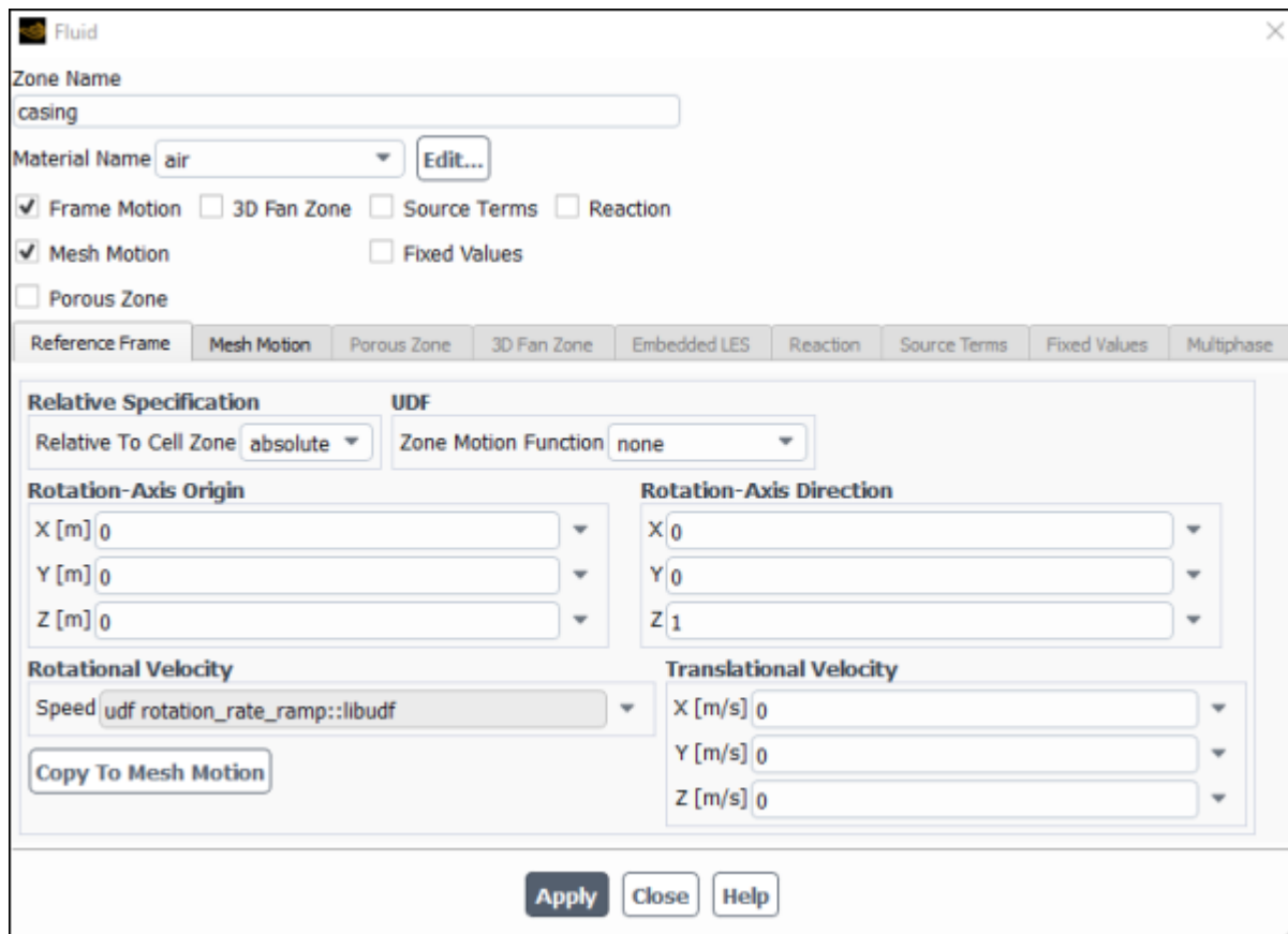
Figure 6.71: The Fluid Dialog Box
