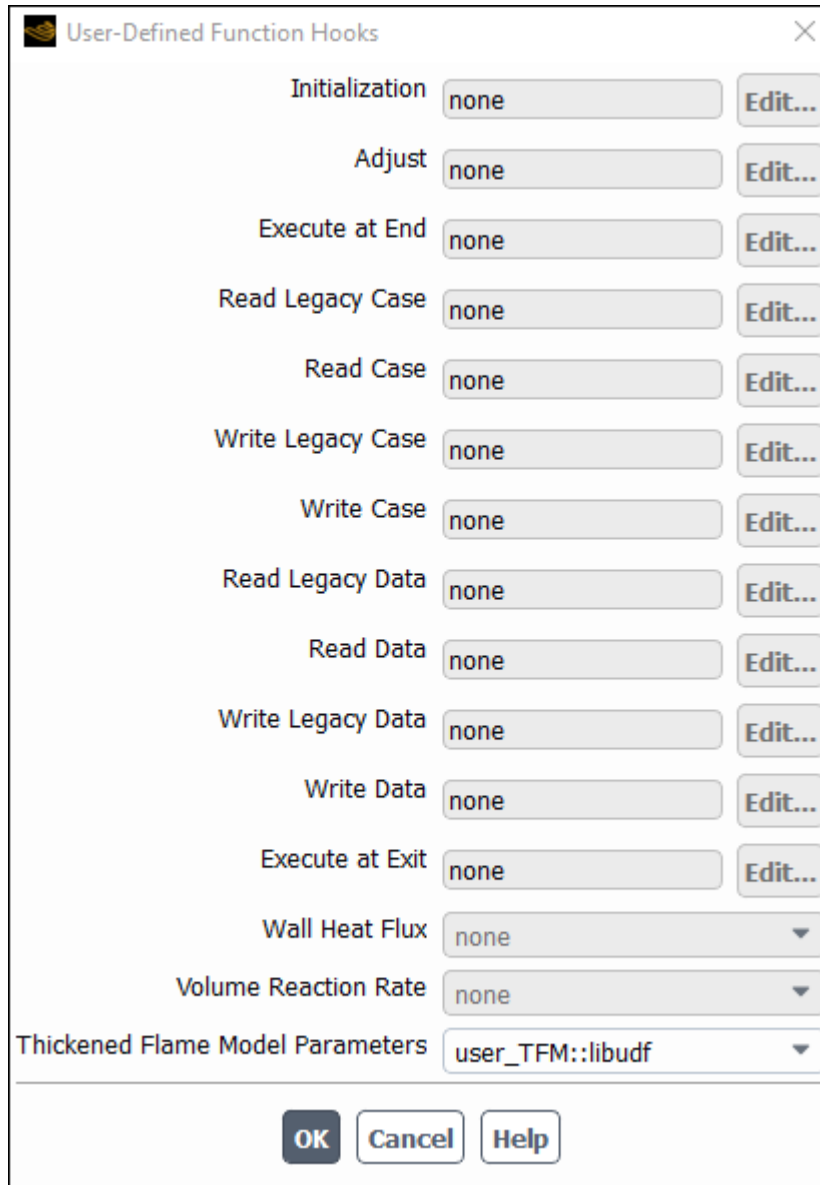
Figure 6.69: The User-Defined Function Hooks Dialog Box
