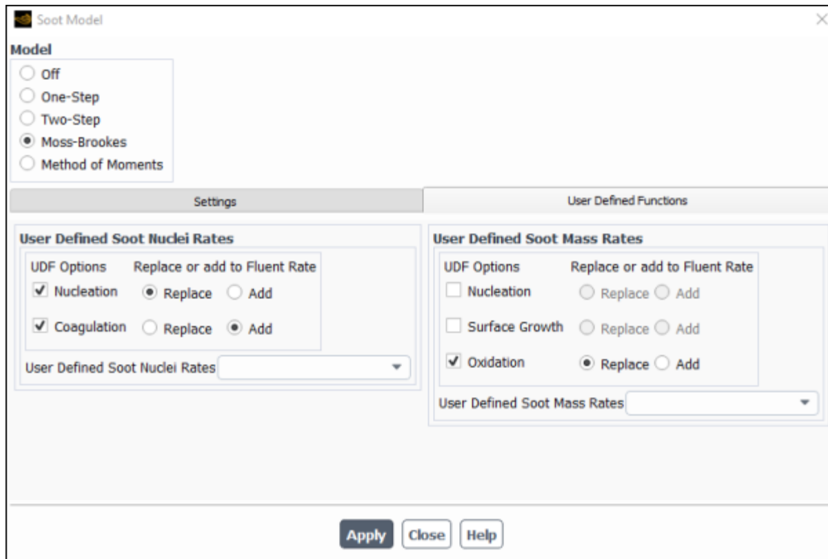
Figure 6.61: The Soot Model Dialog Box (User-Defined Mass and Nucleation Rates)
