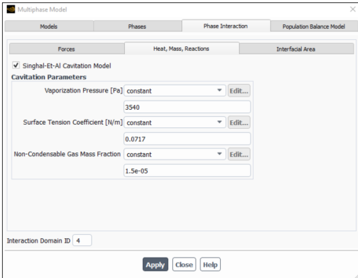
Figure 6.85: The Multiphase Model Dialog Box - Heat, Mass, Reactions Tab
