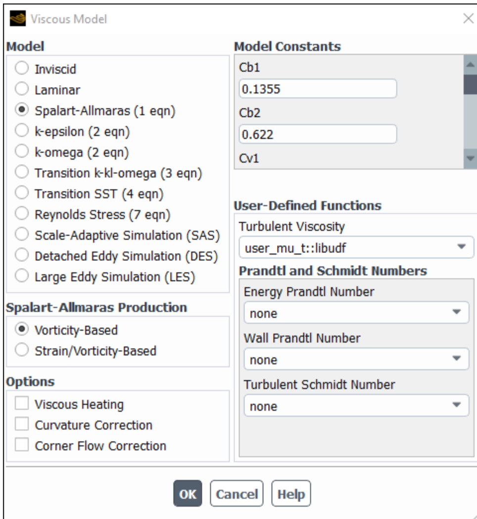
Figure 6.74: The Viscous Model Dialog Box
