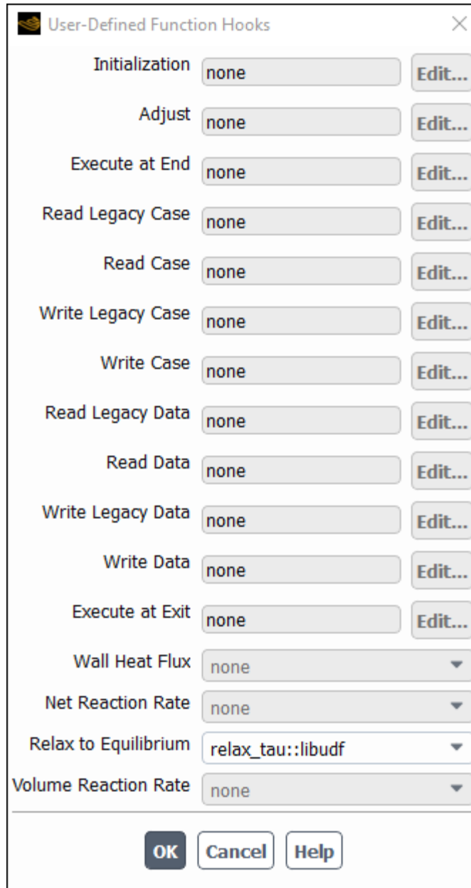
Figure 6.51: The User-Defined Function Hooks Dialog Box
