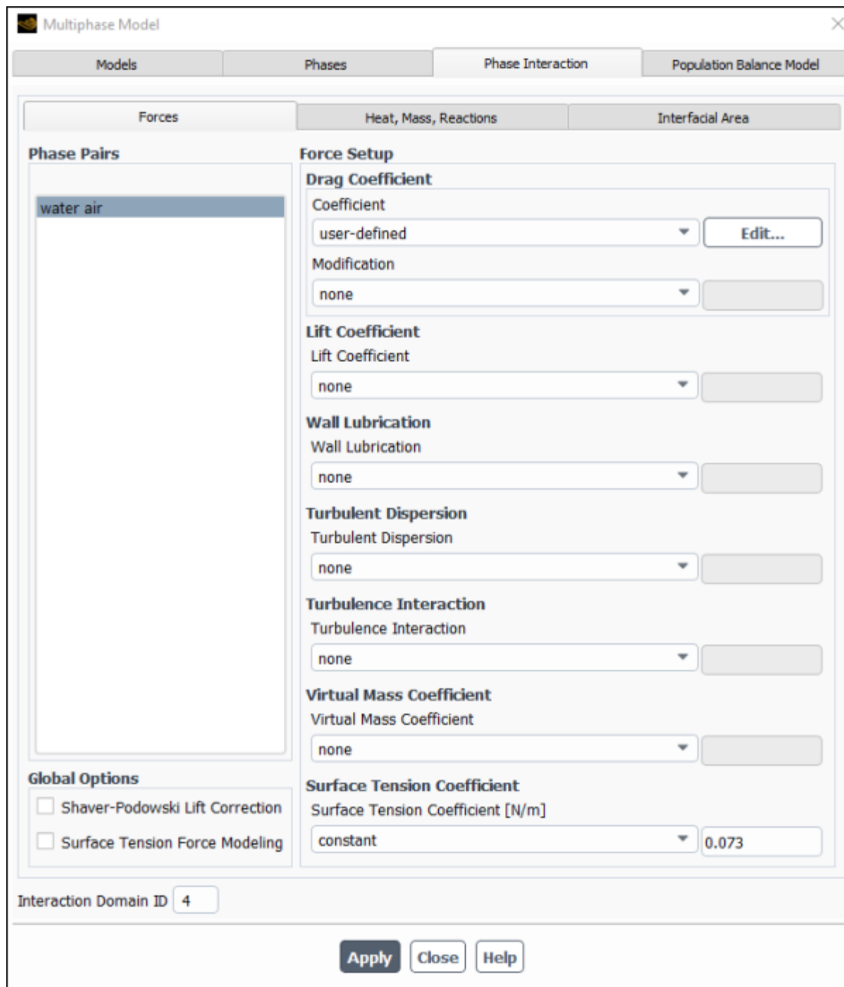
Figure 6.87: The Multiphase Model Dialog Box - Forces Tab
