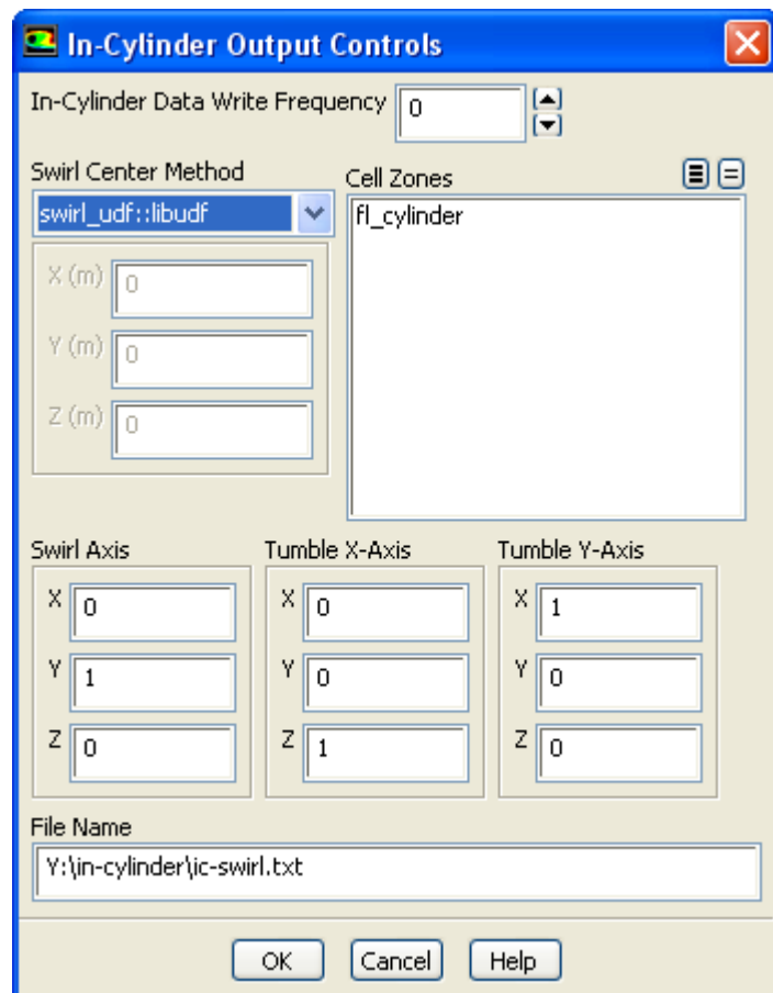
Figure 6.115: In-Cylinder Output Controls Dialog Box
