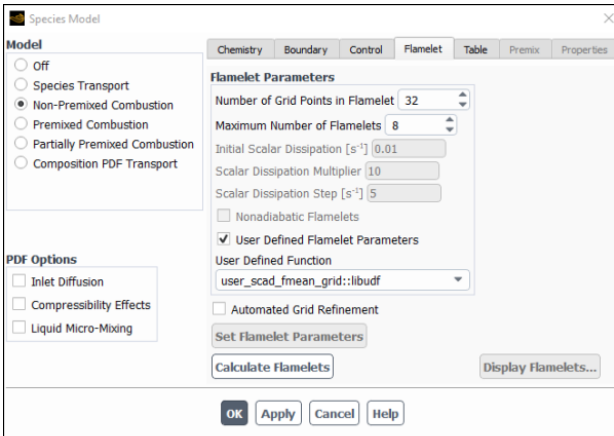
Figure 6.30: The Flamelet Tab Dialog Box (User-Defined Flamelet Parameters)
