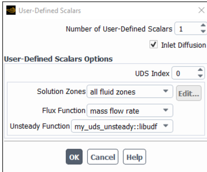
Figure 6.124: The User-Defined Scalars Dialog Box
